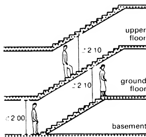
⑦ Superimposed stairs save space
